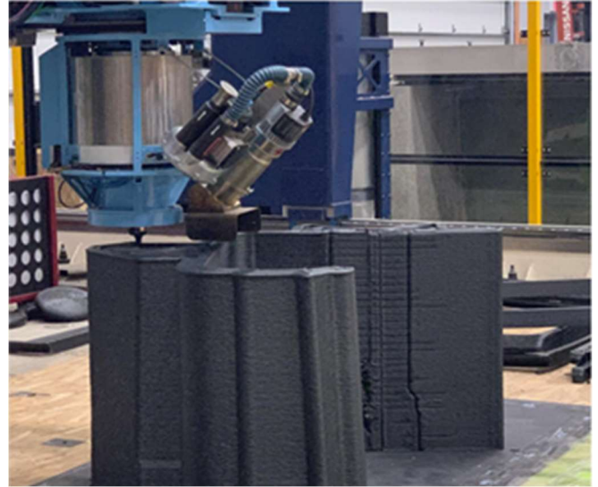
Figure 5.0 Two Large Scale AM molds being printed in one file then separated
